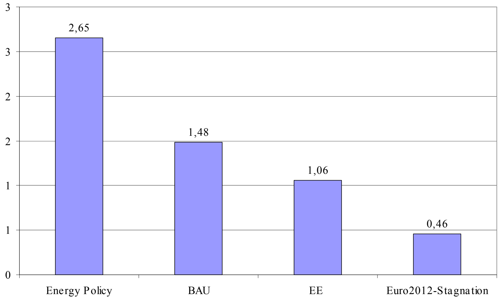
Average increase of electricity consumption in %per year
