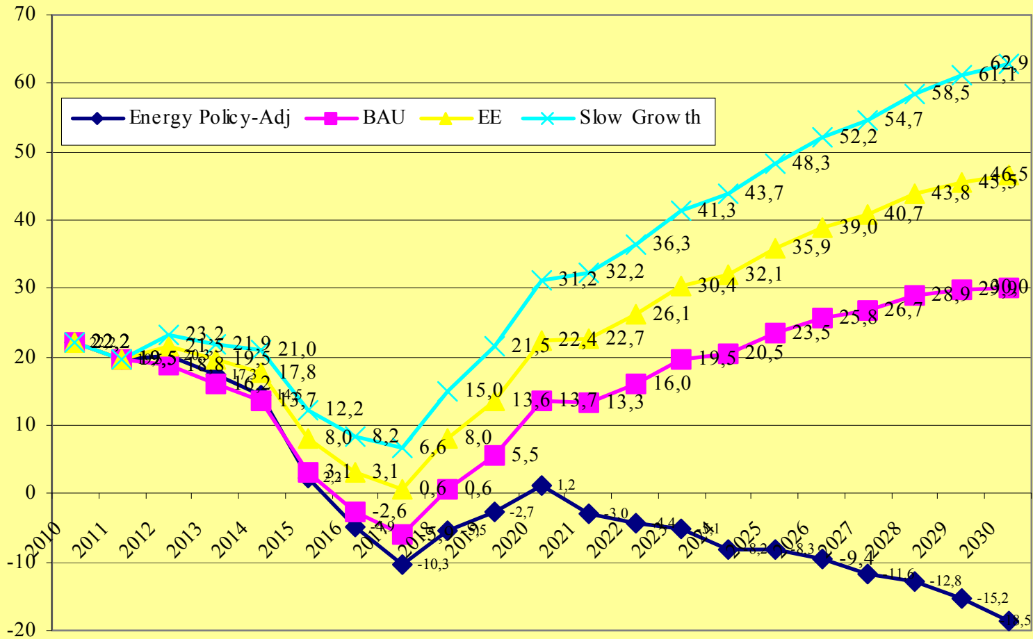
Balance of domestic production and demand in TWh
